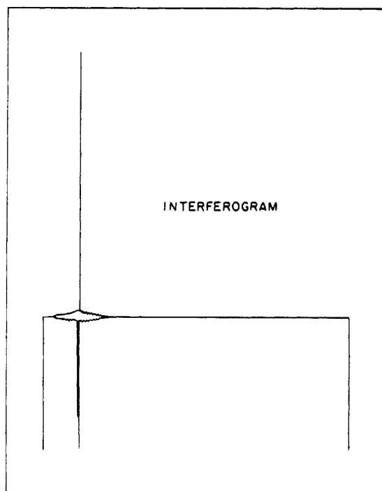
Figure 2. An interferogram.
