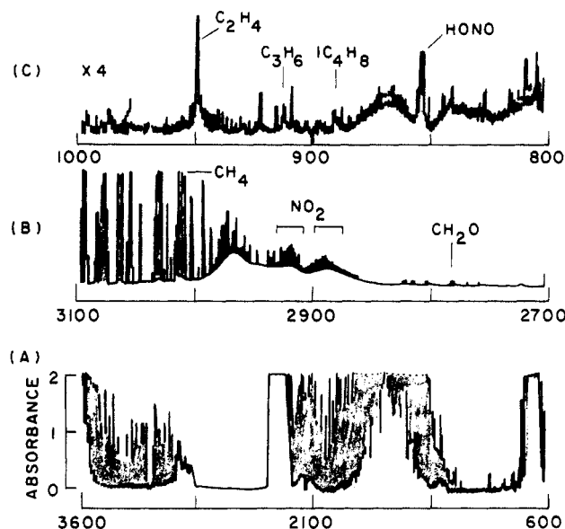
Figure 3. Absorbance spectrum of typical cold-hot cycle, constant volume sampled auto exhaust, at various scale expansions with prominent bands identified (from Figure 6 of ref 5).
